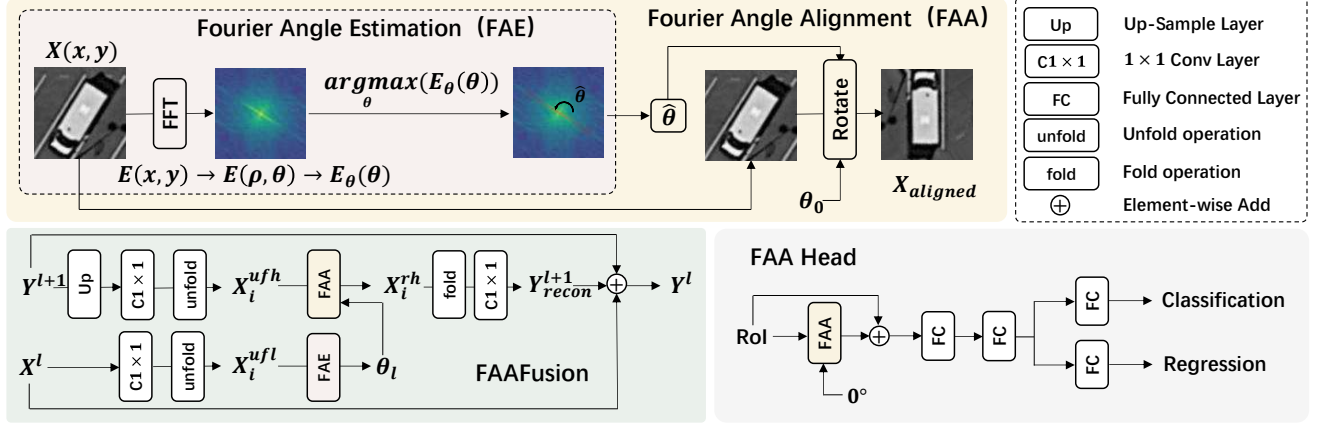
Figure 5. Structures of FAA, FAAFusion and FAA Head. For FAA, it can be divided into two steps. First, we estimate the main direction in frequent domain. And then FAA accepts an external angle and aligns the main direction with it. For FAAFusion, we use the main direction of the lower local feature as the external angle and align the higher local feature with it. For FAA Head, it aligns the main direction of RoI features with 0^\circ to obtain the rotation invariant features.
