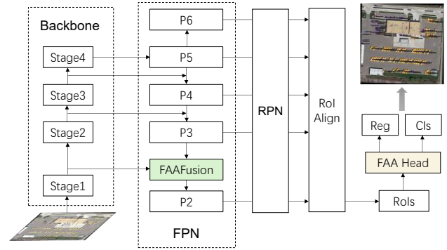
Figure 1. The position of FAAFusion and FAA Head.
