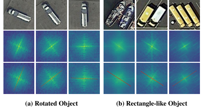
Figure 4. The top row shows the target images in the spatial domain. The second row gives their matching frequency spectra. In the bottom row, red lines point out the main energy directions in each spectrum. (a) If the spatial picture is rotated, its spectrum distribution will be rotated as well. (b) The main spectral direction of one rectangle-like object is perpendicular to the direction of its major axis.
