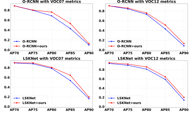
Figure 6. Effectiveness of our method at Oriented R-CNN [44] and LSKNet [25] compared to the original methods on HRSC2016 [33] dataset. In the high IoU threshold range, our method performs better. The AP values are calculated with PASCAL VOC2007 [13] and VOC2012 [14] metrics.
