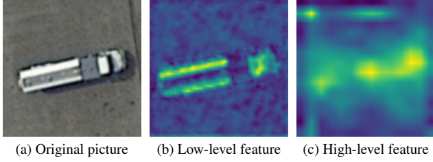
Figure 2. Directional incoherence. High-level feature (c) has strong semantics and large receptive fields but captures the coarse orientation. For example, from (c) we can only infer that the object lies horizontally. Yet many down-samplings blur spatial details, so the orientation signal is low-frequency and vague. Low-level feature (b) keeps rich edges, corners, and textures, giving clear and high-frequency orientation cues.
